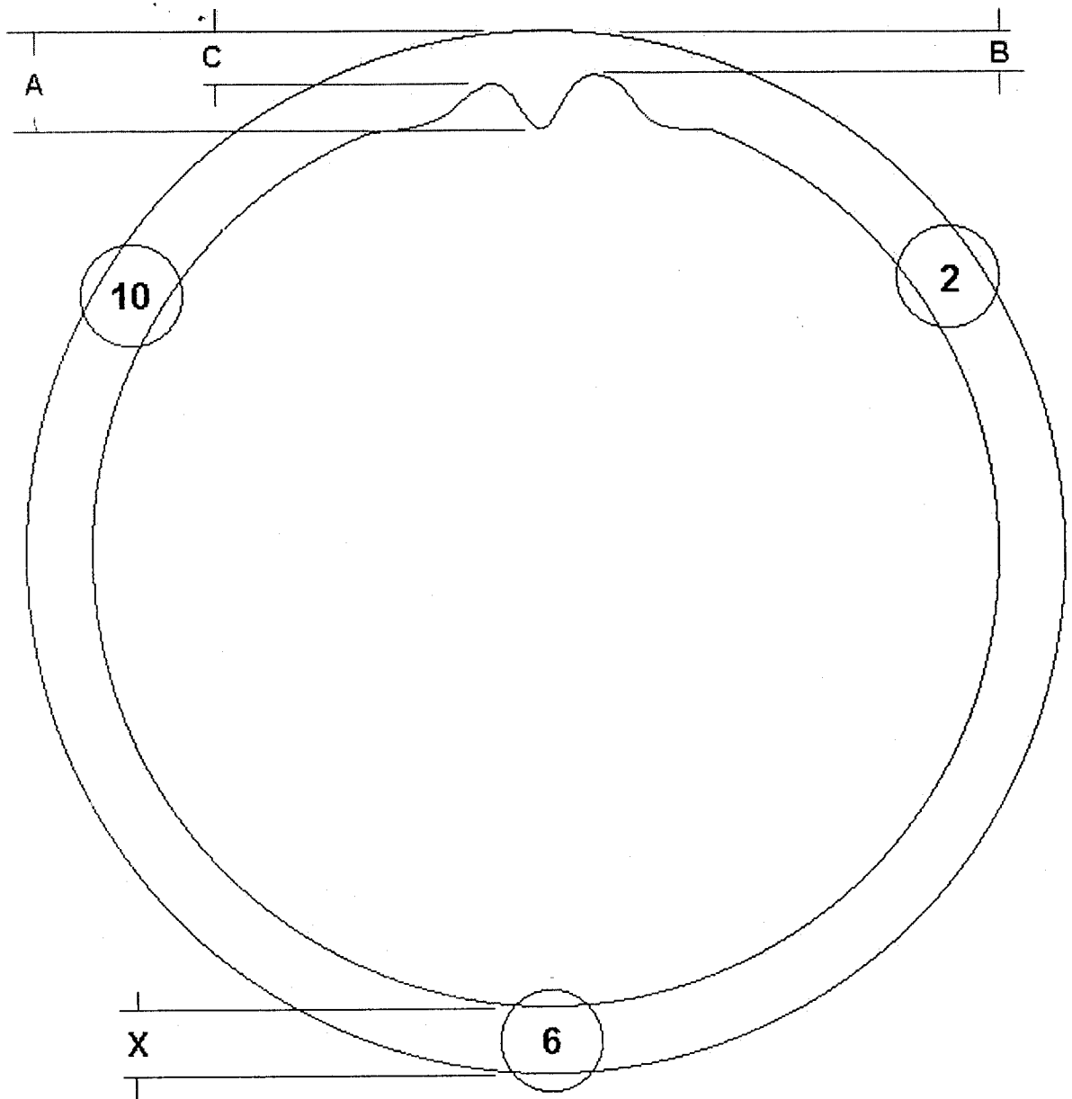
Definition of Tube Measurements
